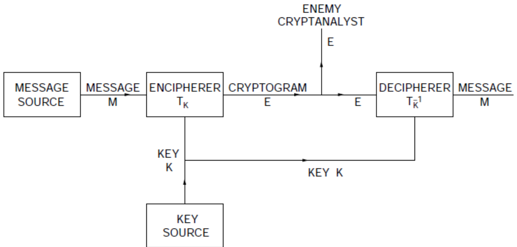
Fig. 1. Schematic of a general secrecy system
